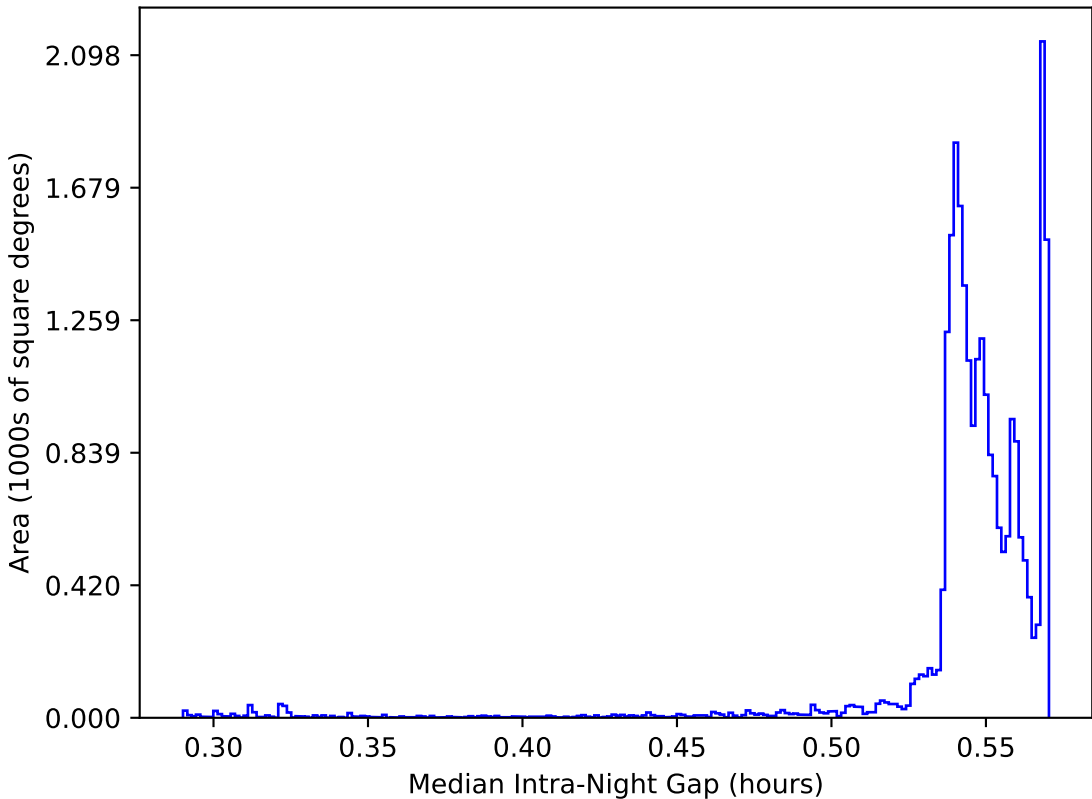
too_elab_r16_d3_griz_v3.4_10yrs All sky: Median Intra-Night Gap
