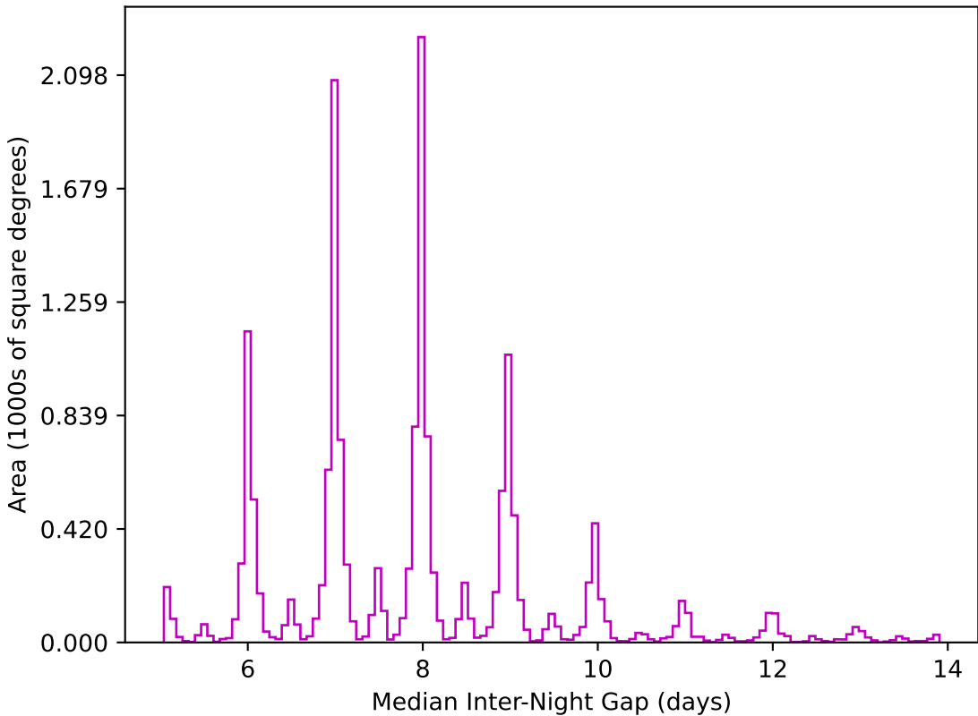
too_elab_r16_d3_griz_v3.4_10yrs WFD z band: Median Inter-Night Gap
