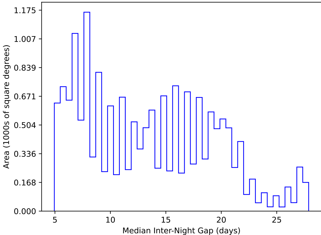
too_elab_r16_d3_griz_v3.4_10yrs WFD y band: Median Inter-Night Gap
