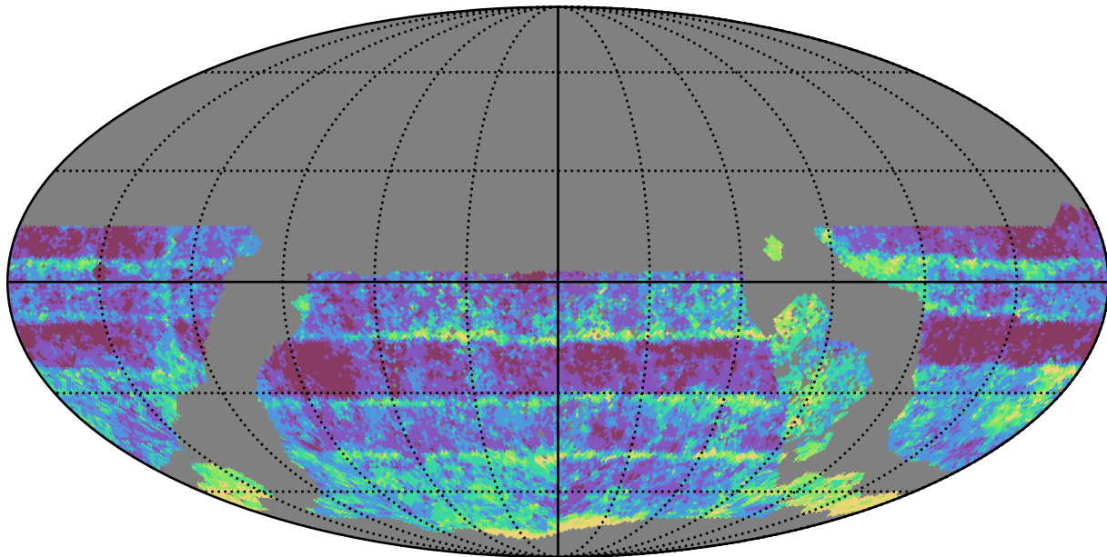
too_elab_r16_d3_griz_v3.4_10yrs WFD r band: Median Inter-Night Gap
