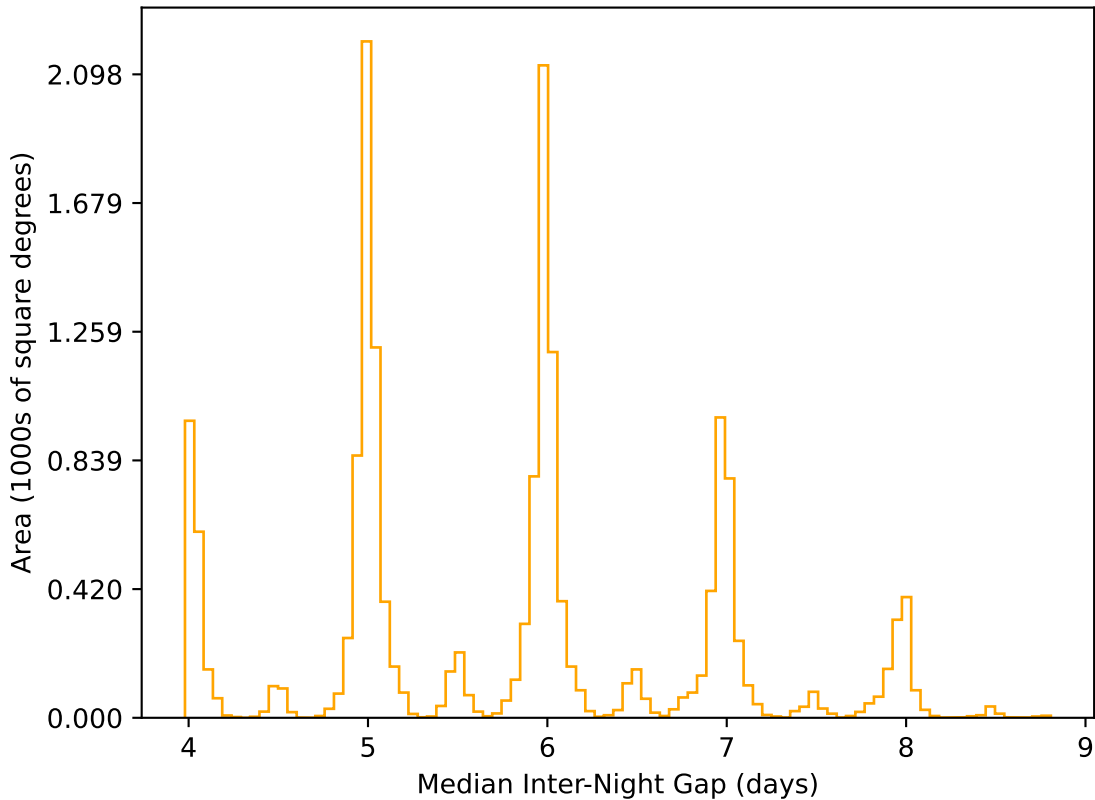
too_elab_r16_d3_griz_v3.4_10yrs WFD r band: Median Inter-Night Gap
