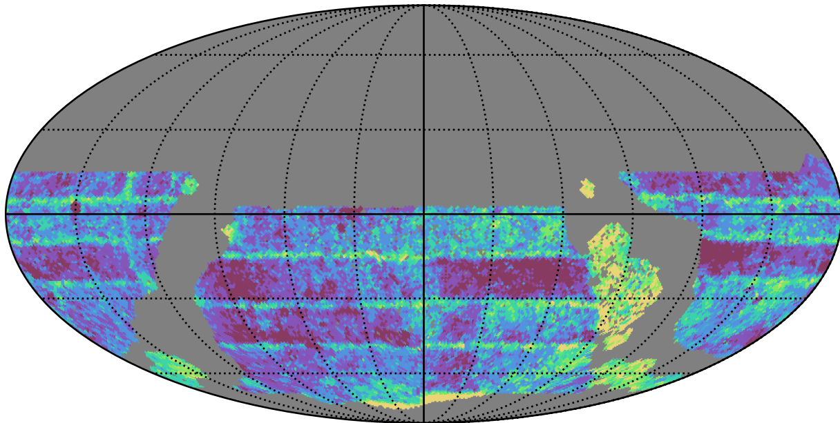
too_elab_r16_d3_griz_v3.4_10yrs WFD i band: Median Inter-Night Gap
