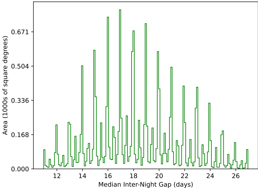
too_elab_r16_d3_griz_v3.4_10yrs WFD g band: Median Inter-Night Gap
