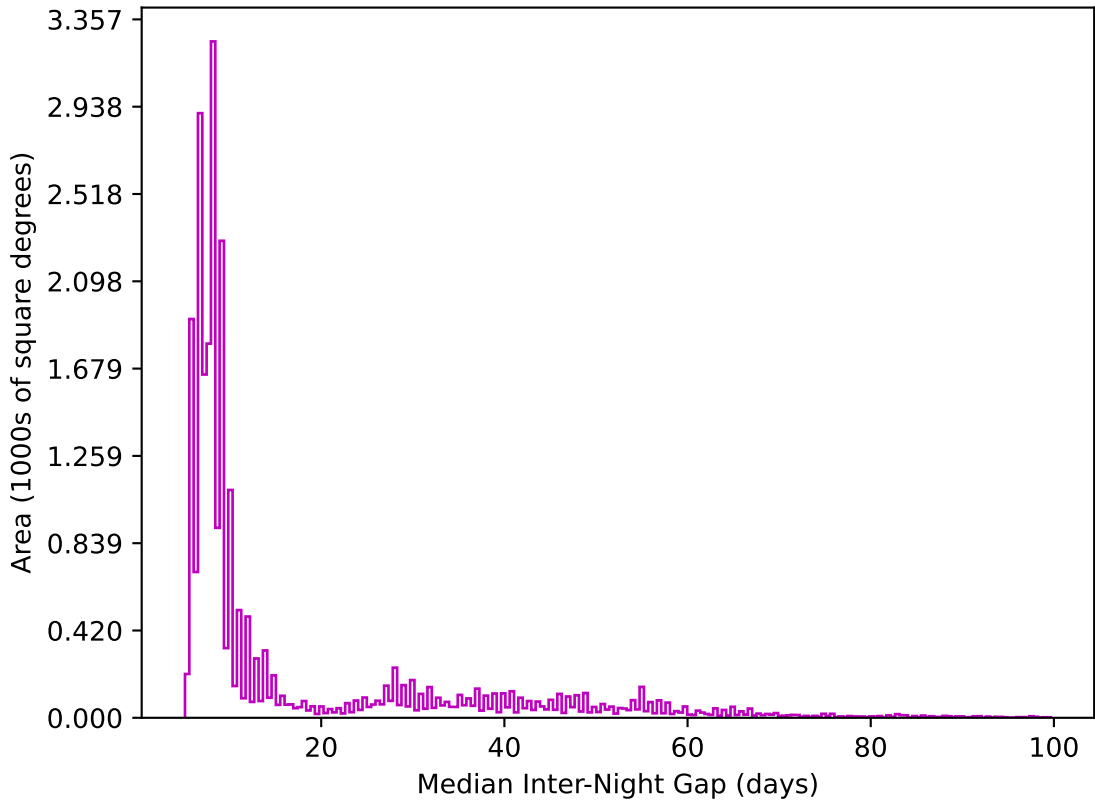
too_elab_r16_d3_griz_v3.4_10yrs All sky z band: Median Inter-Night Gap
