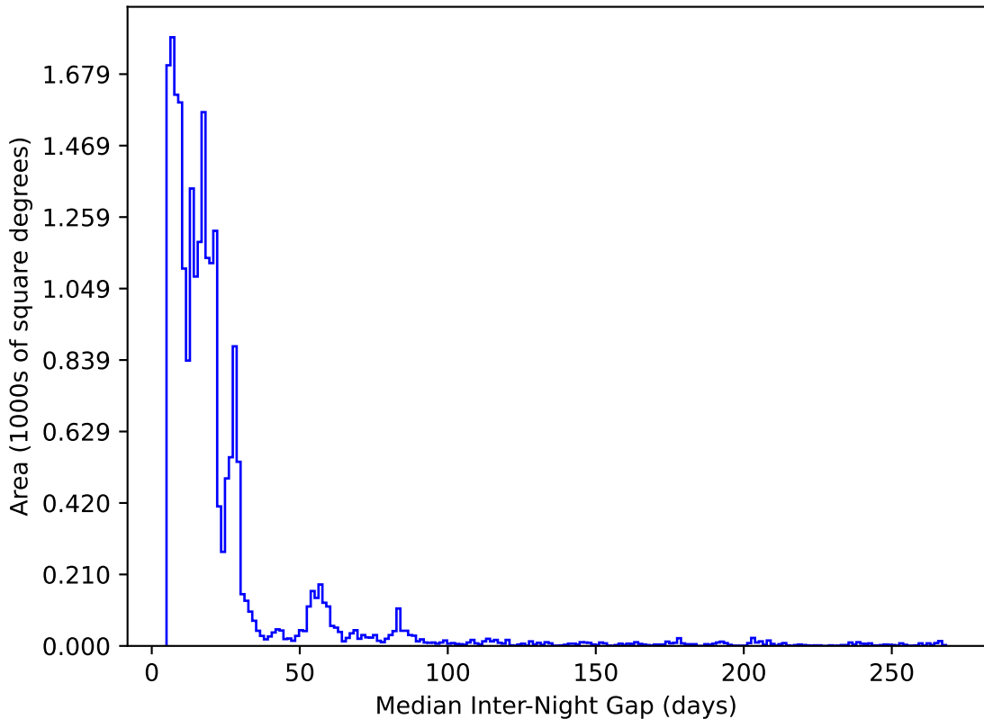
too_elab_r16_d3_griz_v3.4_10yrs All sky y band: Median Inter-Night Gap
