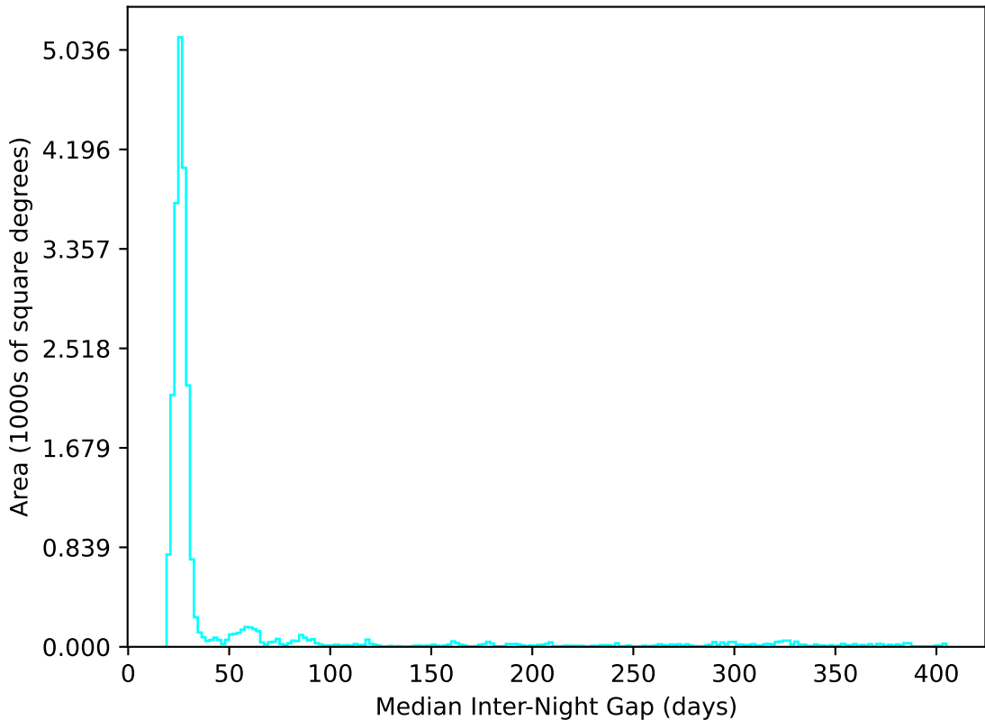
too_elab_r16_d3_griz_v3.4_10yrs All sky u band: Median Inter-Night Gap
