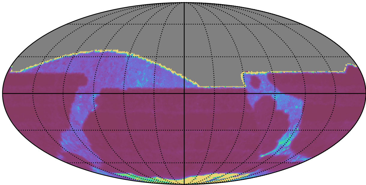
too_elab_r16_d3_griz_v3.4_10yrs All sky r band: Median Inter-Night Gap
