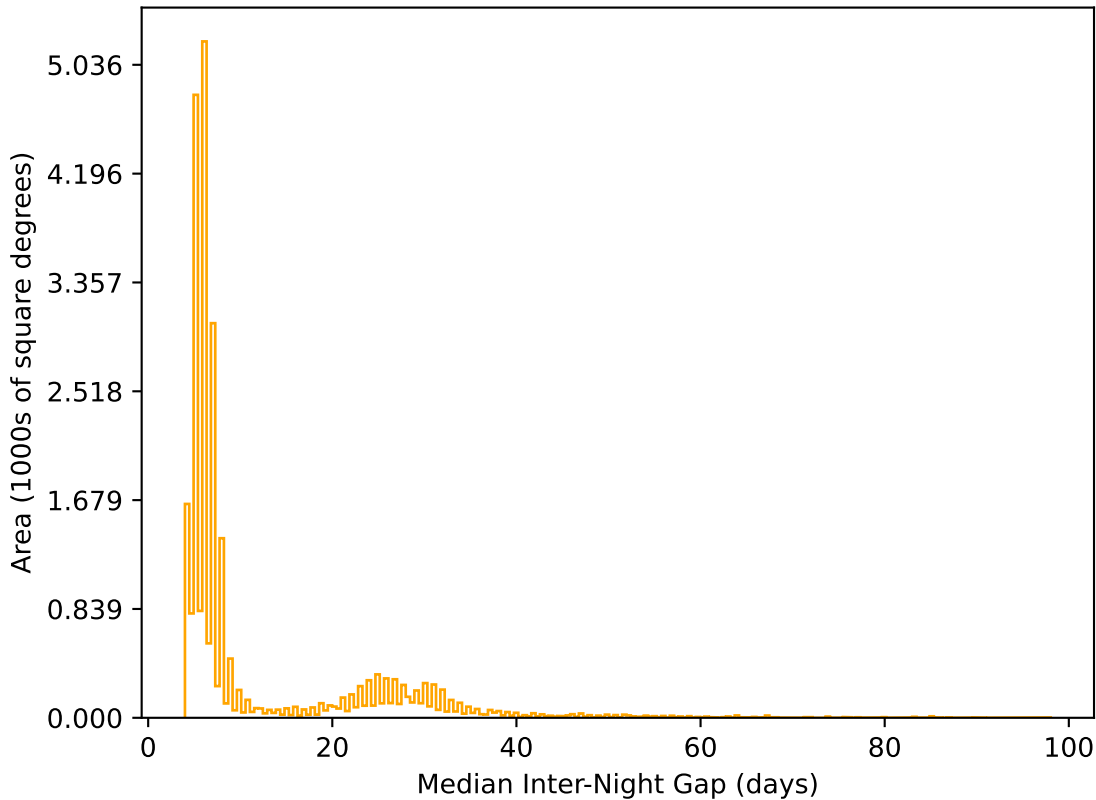
too_elab_r16_d3_griz_v3.4_10yrs All sky r band: Median Inter-Night Gap
