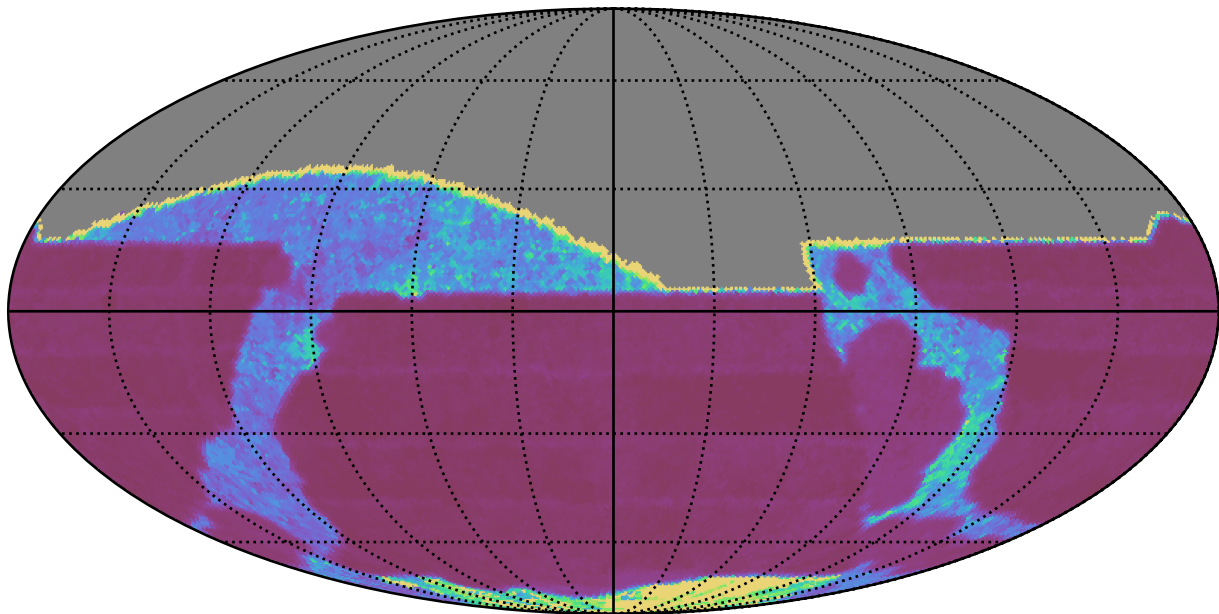
too_elab_r16_d3_griz_v3.4_10yrs All sky i band: Median Inter-Night Gap
