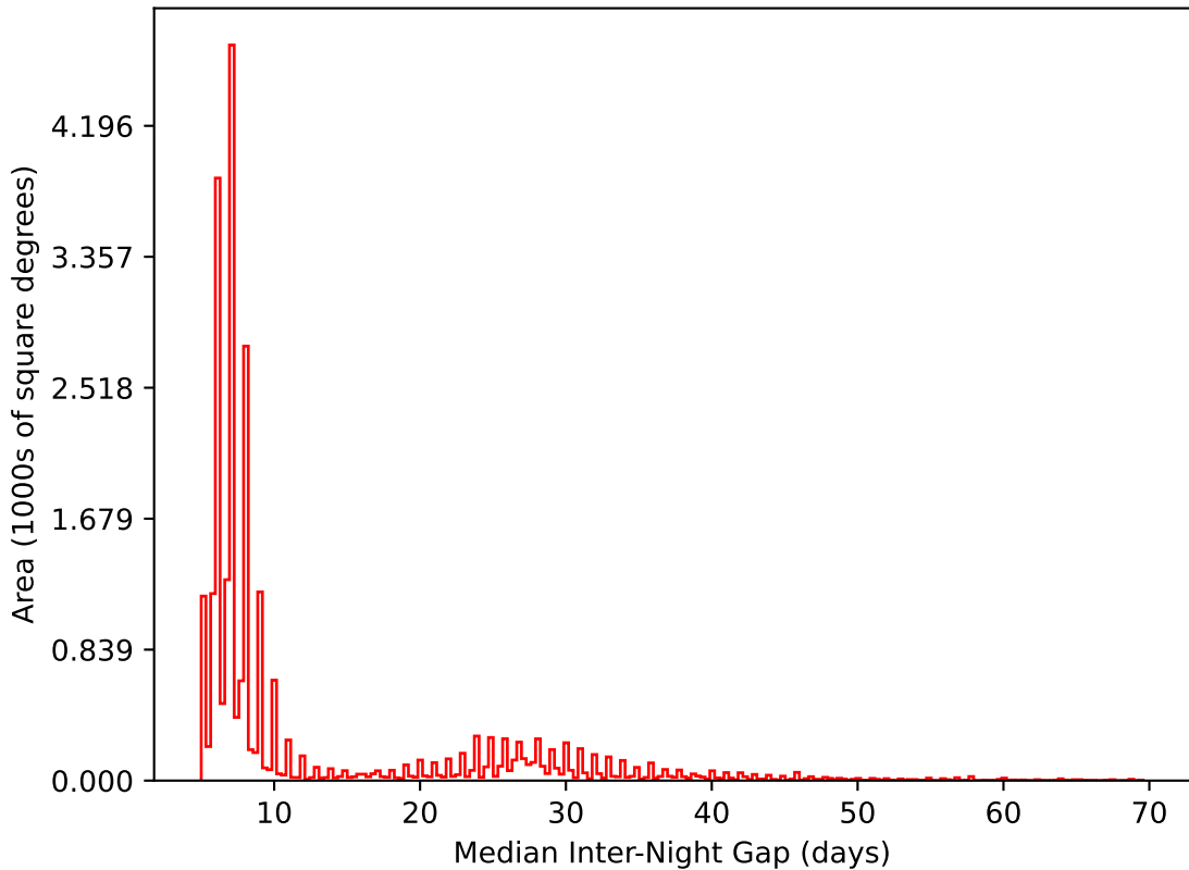
too_elab_r16_d3_griz_v3.4_10yrs All sky i band: Median Inter-Night Gap
