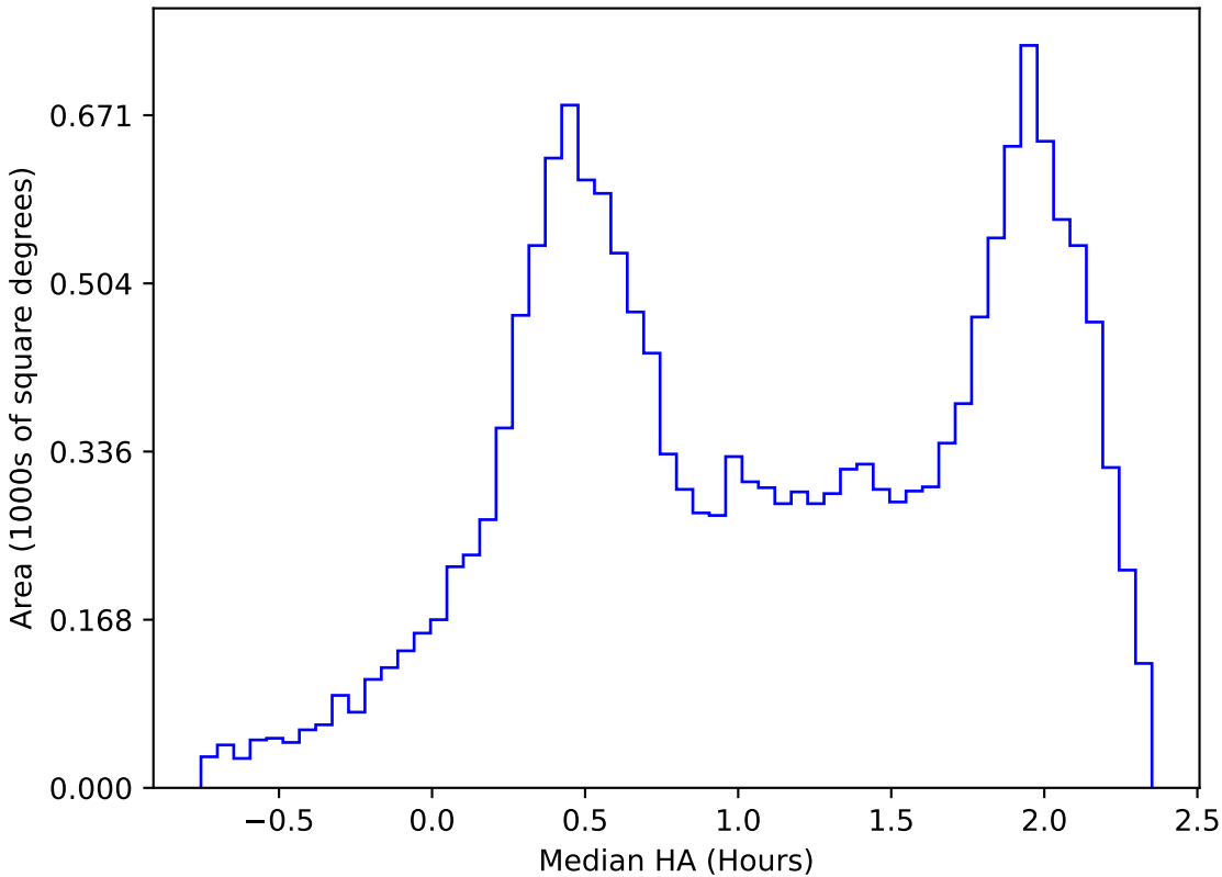
too_elab_r16_d3_griz_v3.4_10yrs WFD z band: Median HA
