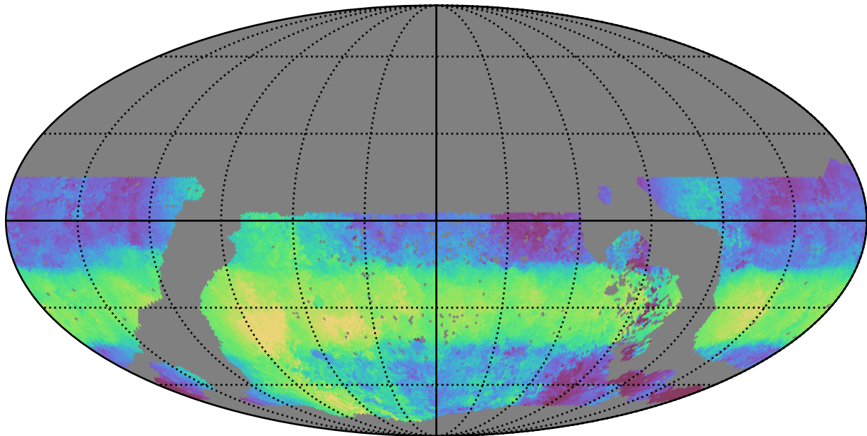
too_elab_r16_d3_griz_v3.4_10yrs WFD u band: Median HA
