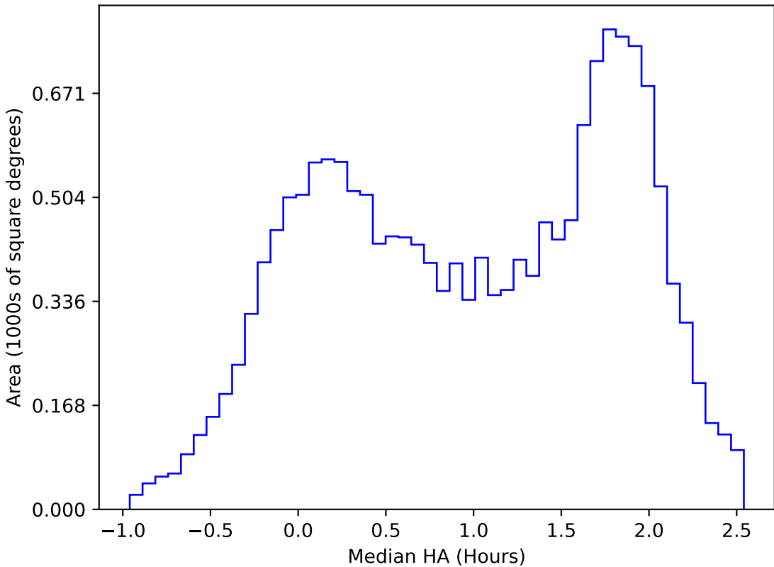
too_elab_r16_d3_griz_v3.4_10yrs WFD u band: Median HA
