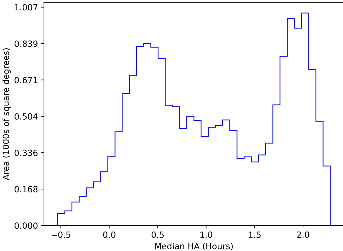
too_elab_r16_d3_griz_v3.4_10yrs WFD i band: Median HA
