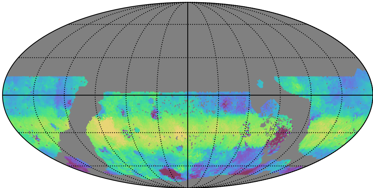
too_elab_r16_d3_griz_v3.4_10yrs WFD g band: Median HA
