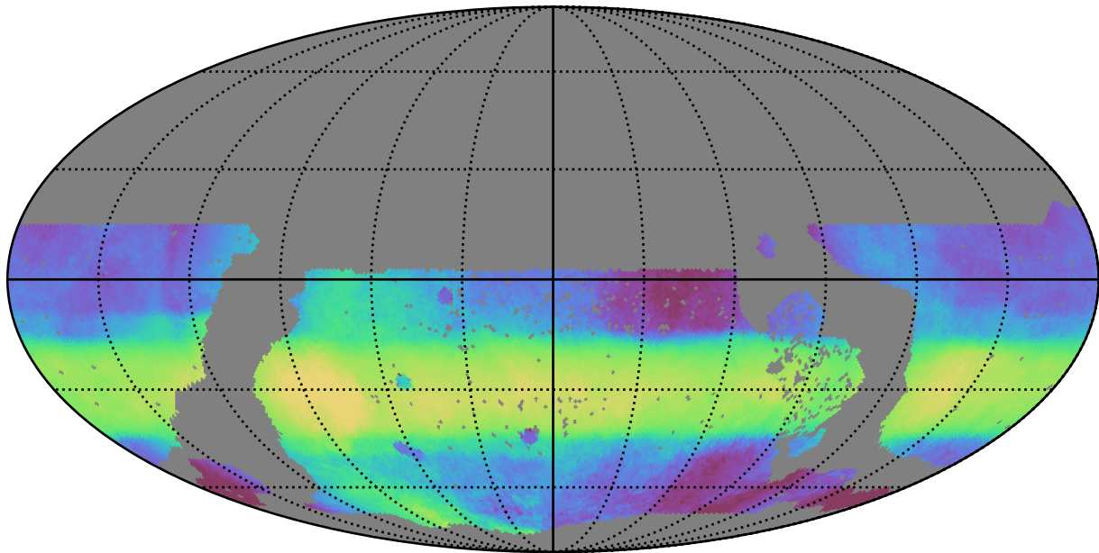
too_elab_r16_d3_griz_v3.4_10yrs WFD all bands: Median HA
