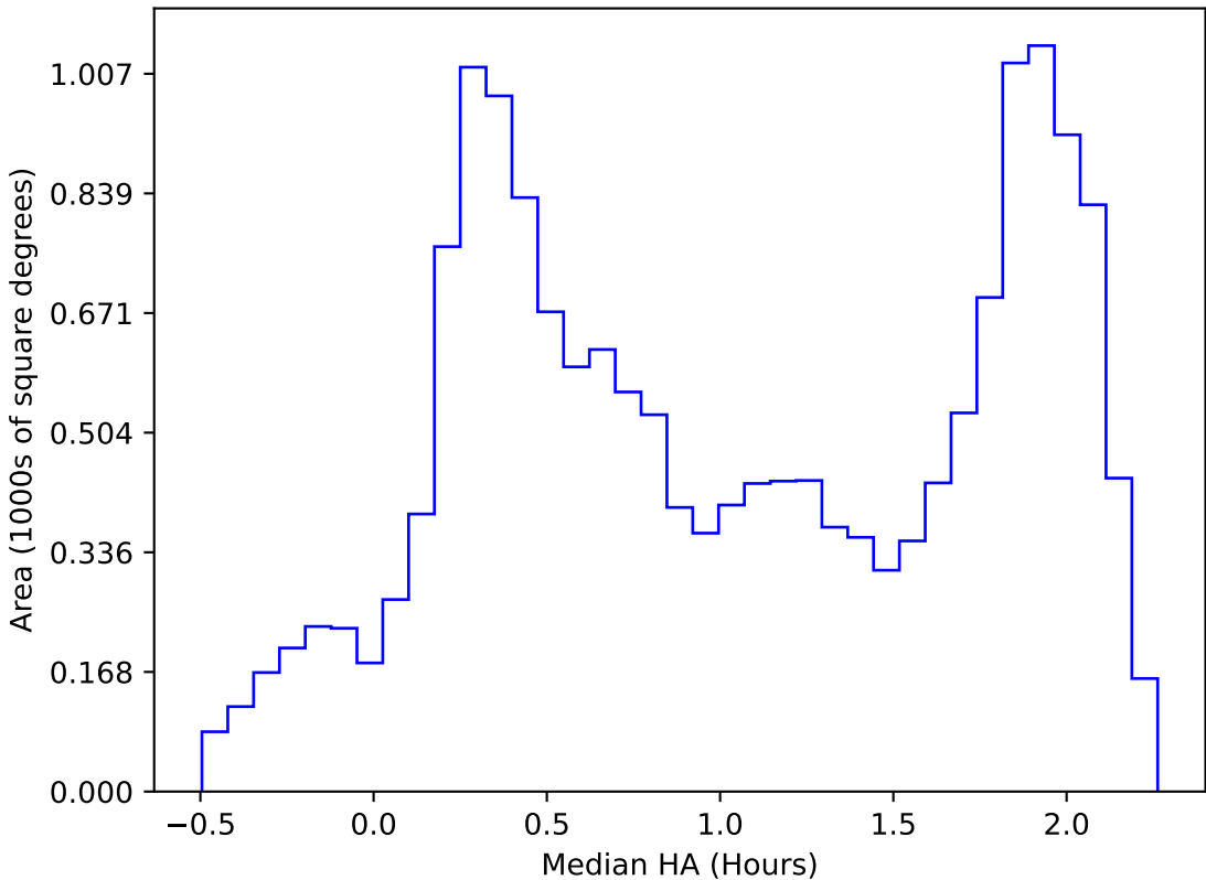
too_elab_r16_d3_griz_v3.4_10yrs WFD all bands: Median HA
