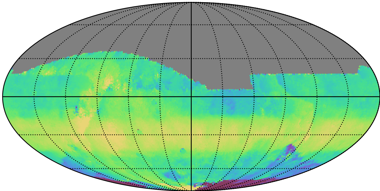
too_elab_r16_d3_griz_v3.4_10yrs All sky z band: Median HA
