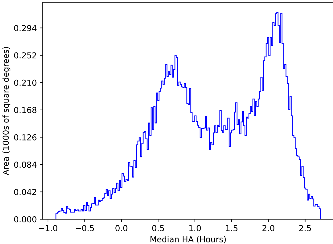
too_elab_r16_d3_griz_v3.4_10yrs All sky y band: Median HA
