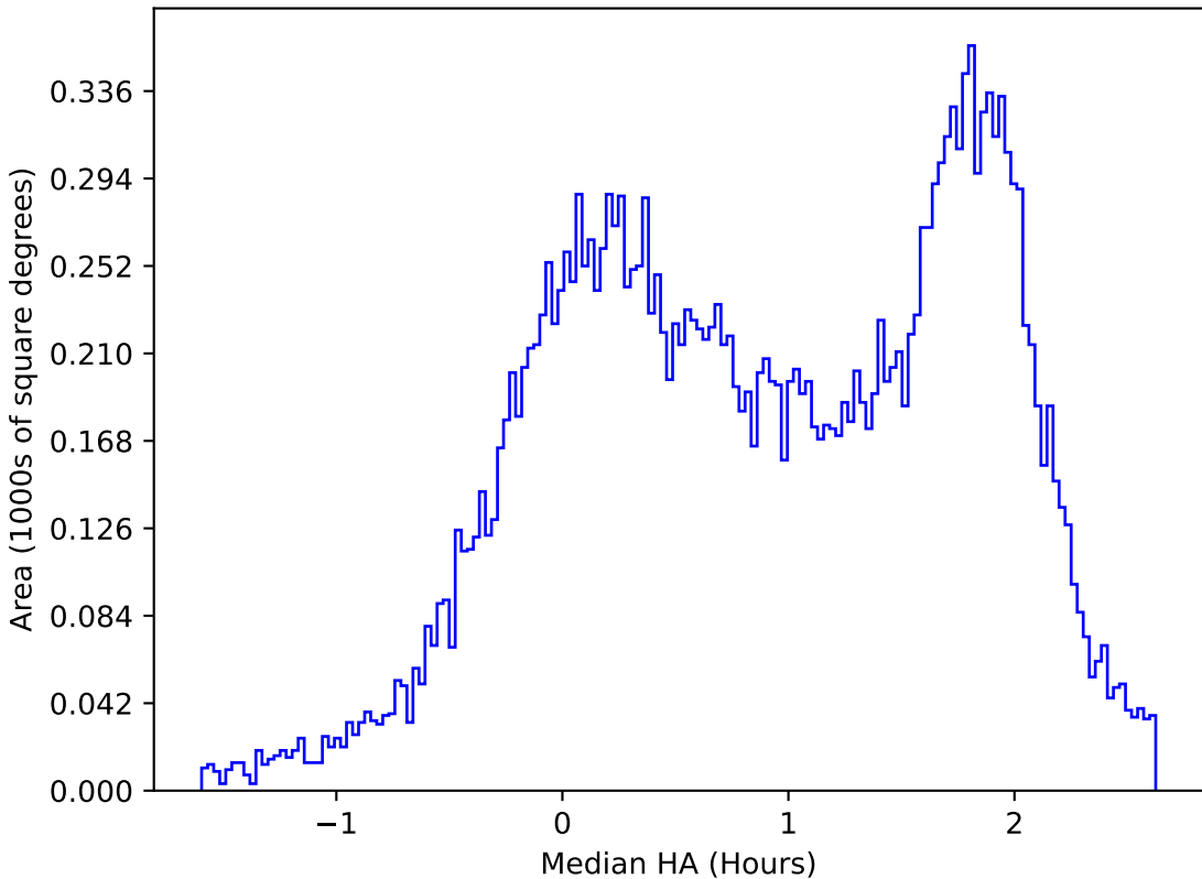
too_elab_r16_d3_griz_v3.4_10yrs All sky u band: Median HA
