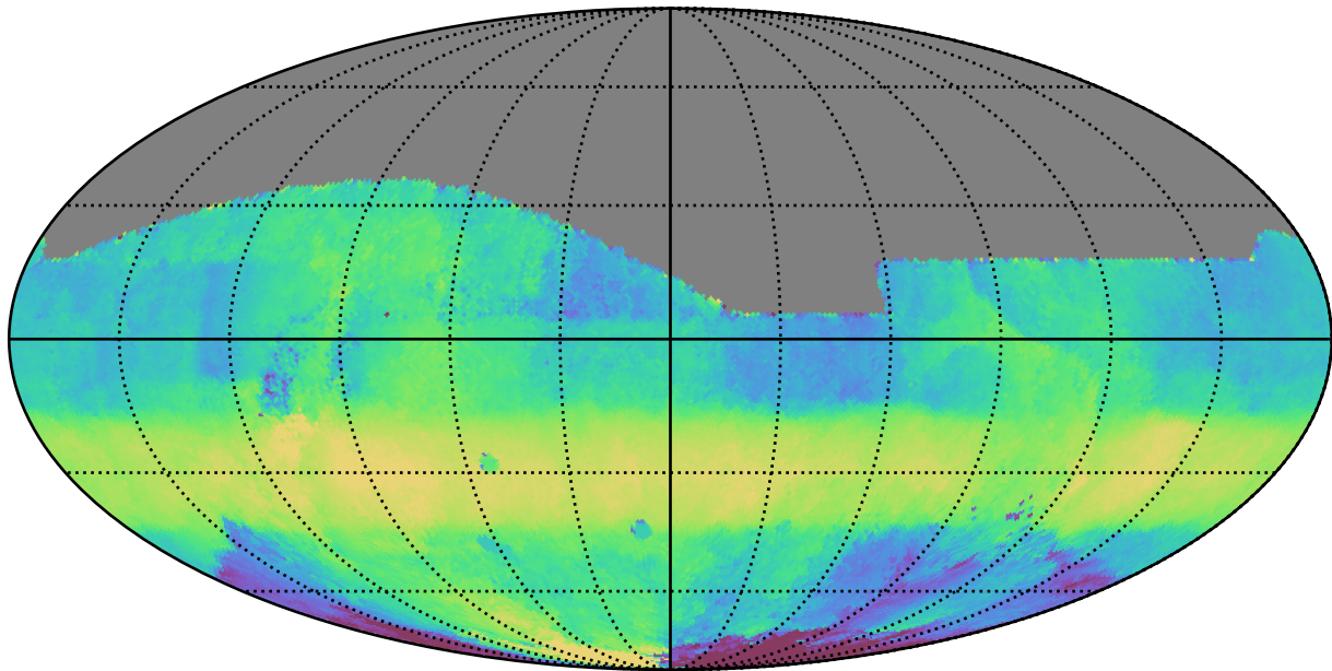
too_elab_r16_d3_griz_v3.4_10yrs All sky r band: Median HA
