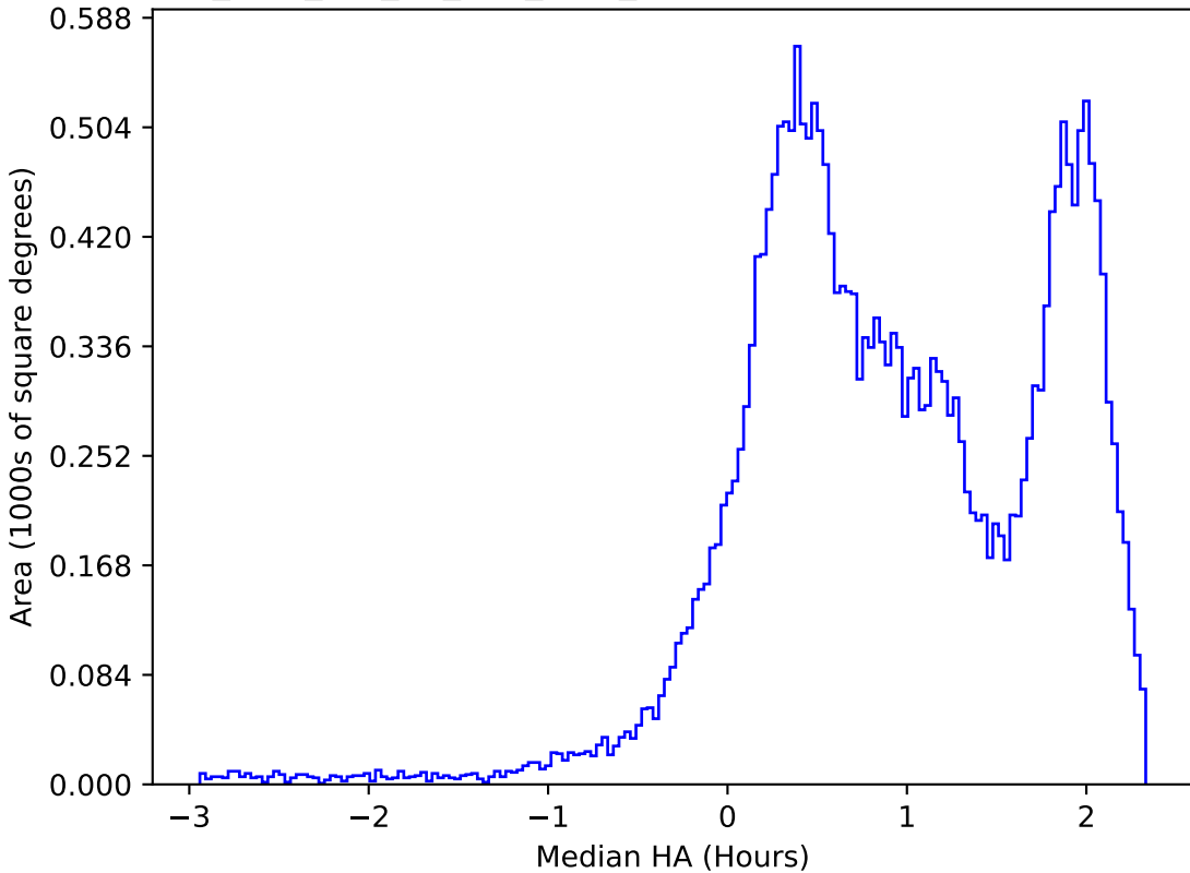
too_elab_r16_d3_griz_v3.4_10yrs All sky i band: Median HA
