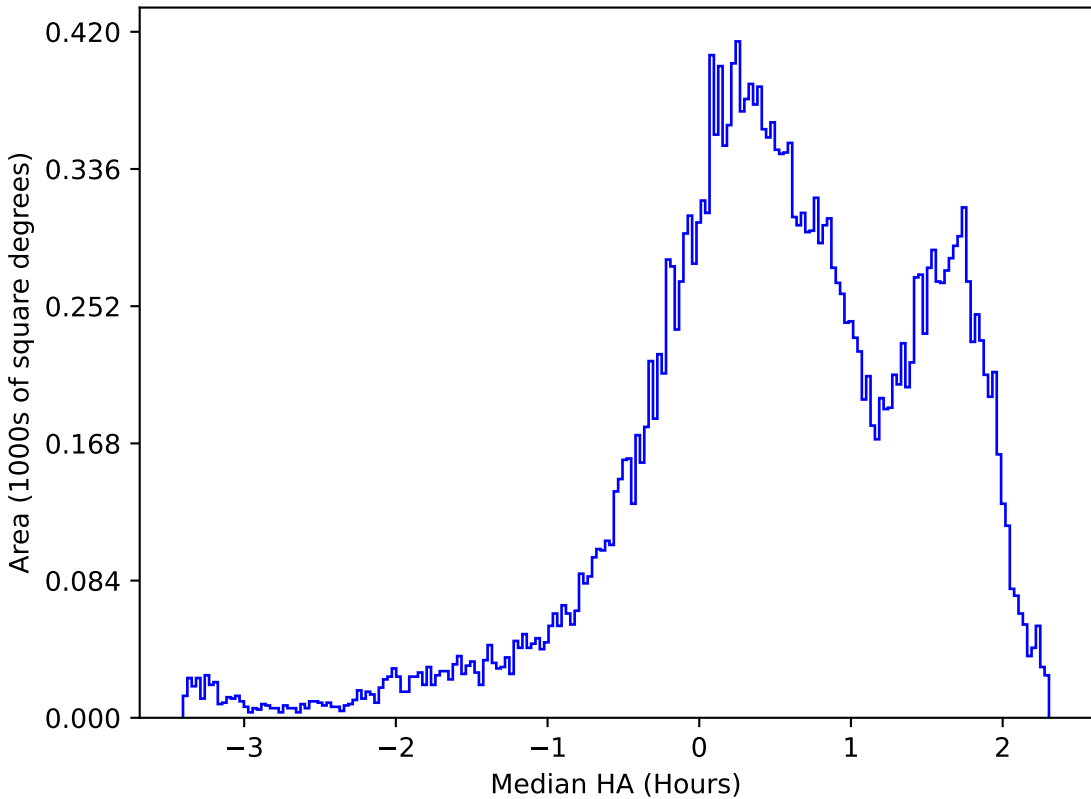
too_elab_r16_d3_griz_v3.4_10yrs All sky g band: Median HA
