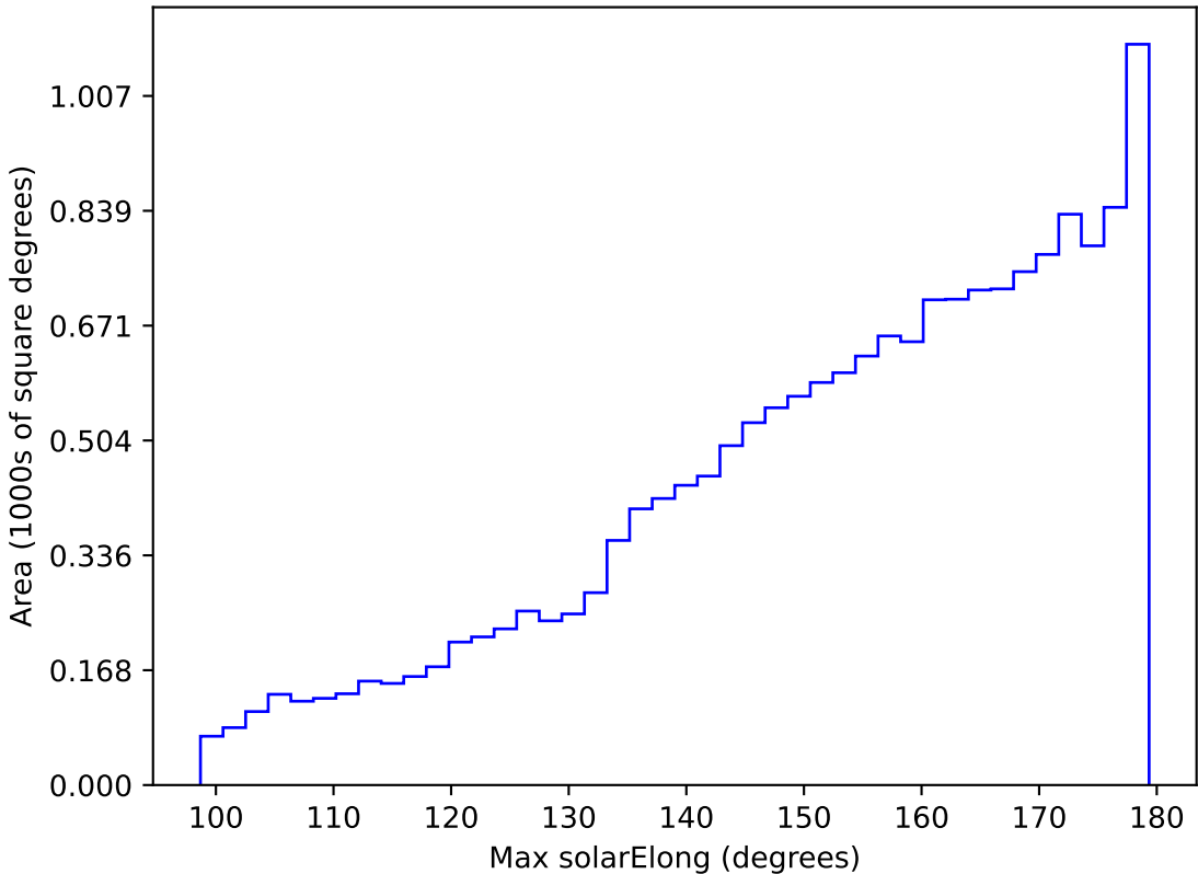
too_elab_r16_d3_griz_v3.4_10yrs WFD z band: Max solarElong
