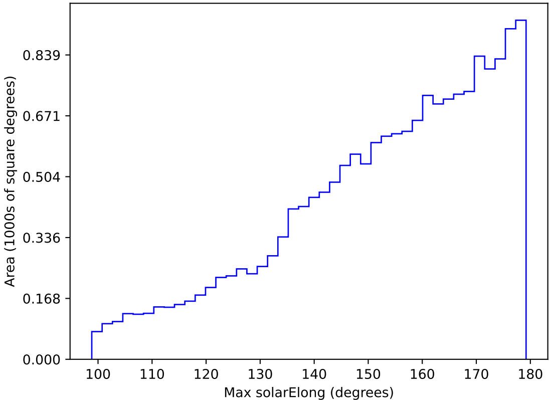
too_elab_r16_d3_griz_v3.4_10yrs WFD y band: Max solarElong
