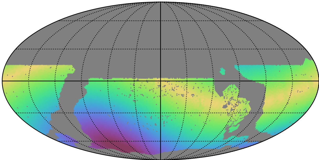
too_elab_r16_d3_griz_v3.4_10yrs WFD u band: Max solarElong
