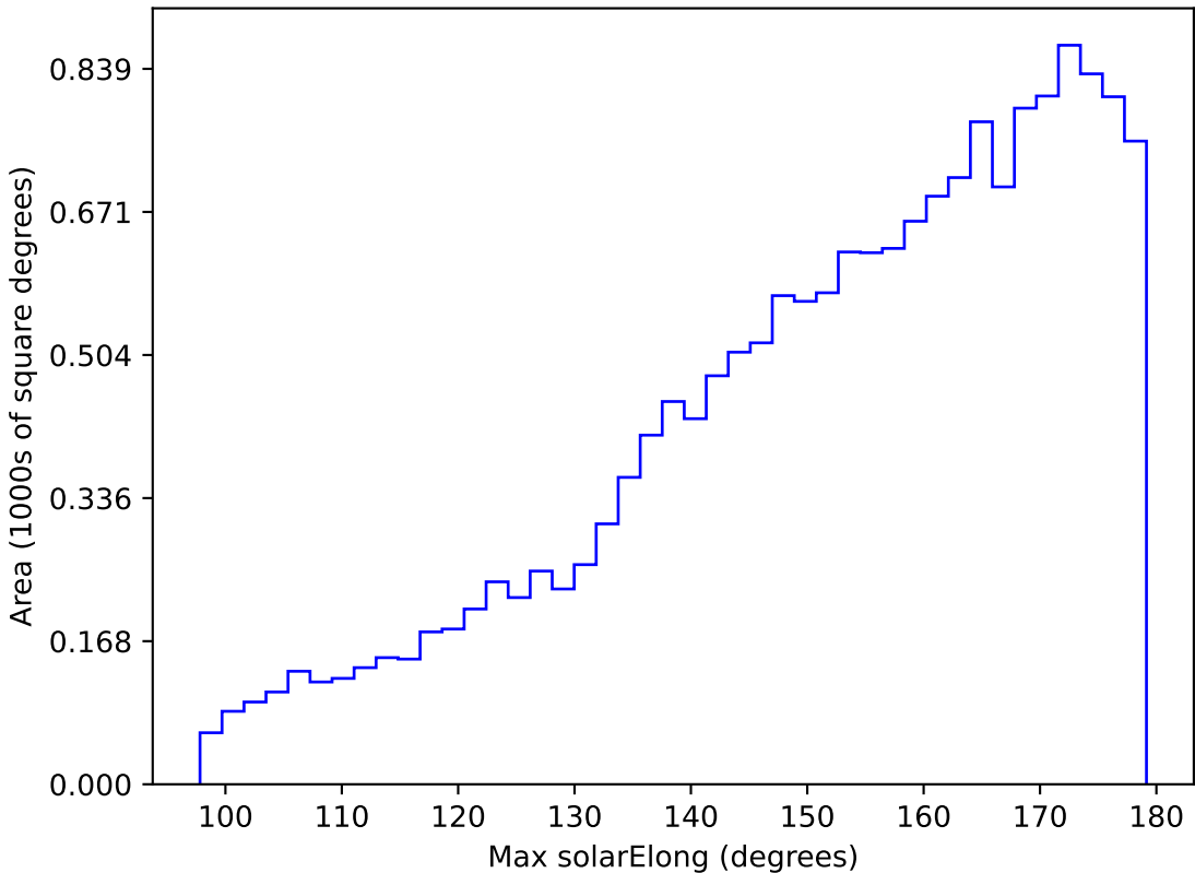
too_elab_r16_d3_griz_v3.4_10yrs WFD u band: Max solarElong
