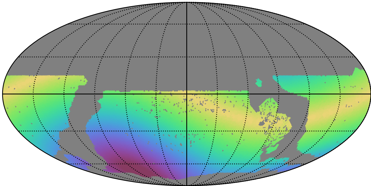
too_elab_r16_d3_griz_v3.4_10yrs WFD r band: Max solarElong
