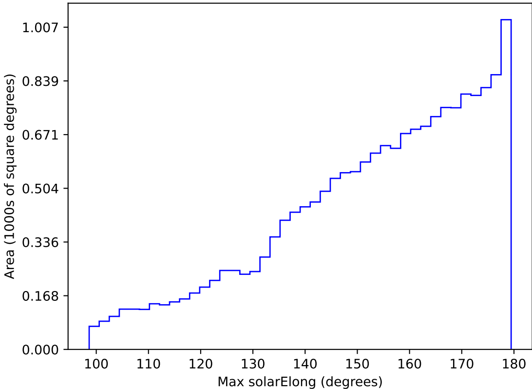
too_elab_r16_d3_griz_v3.4_10yrs WFD r band: Max solarElong
