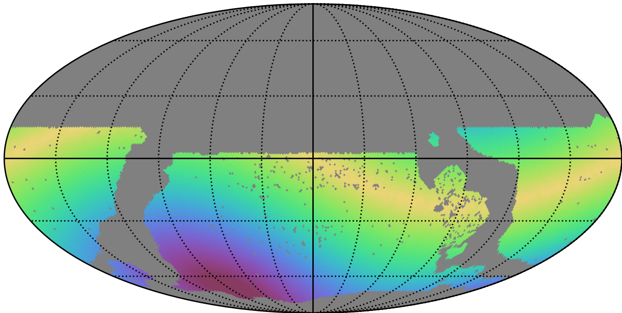
too_elab_r16_d3_griz_v3.4_10yrs WFD i band: Max solarElong
