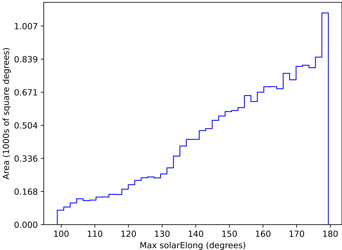
too_elab_r16_d3_griz_v3.4_10yrs WFD i band: Max solarElong
