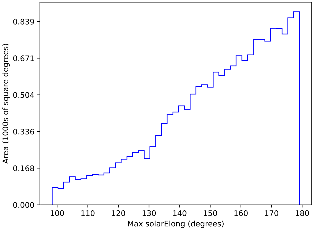
too_elab_r16_d3_griz_v3.4_10yrs WFD g band: Max solarElong
