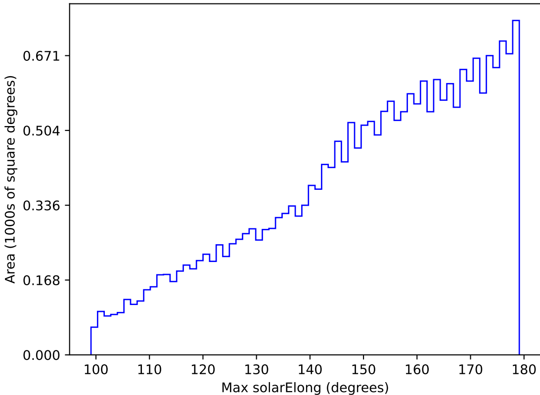
too_elab_r16_d3_griz_v3.4_10yrs All sky y band: Max solarElong
