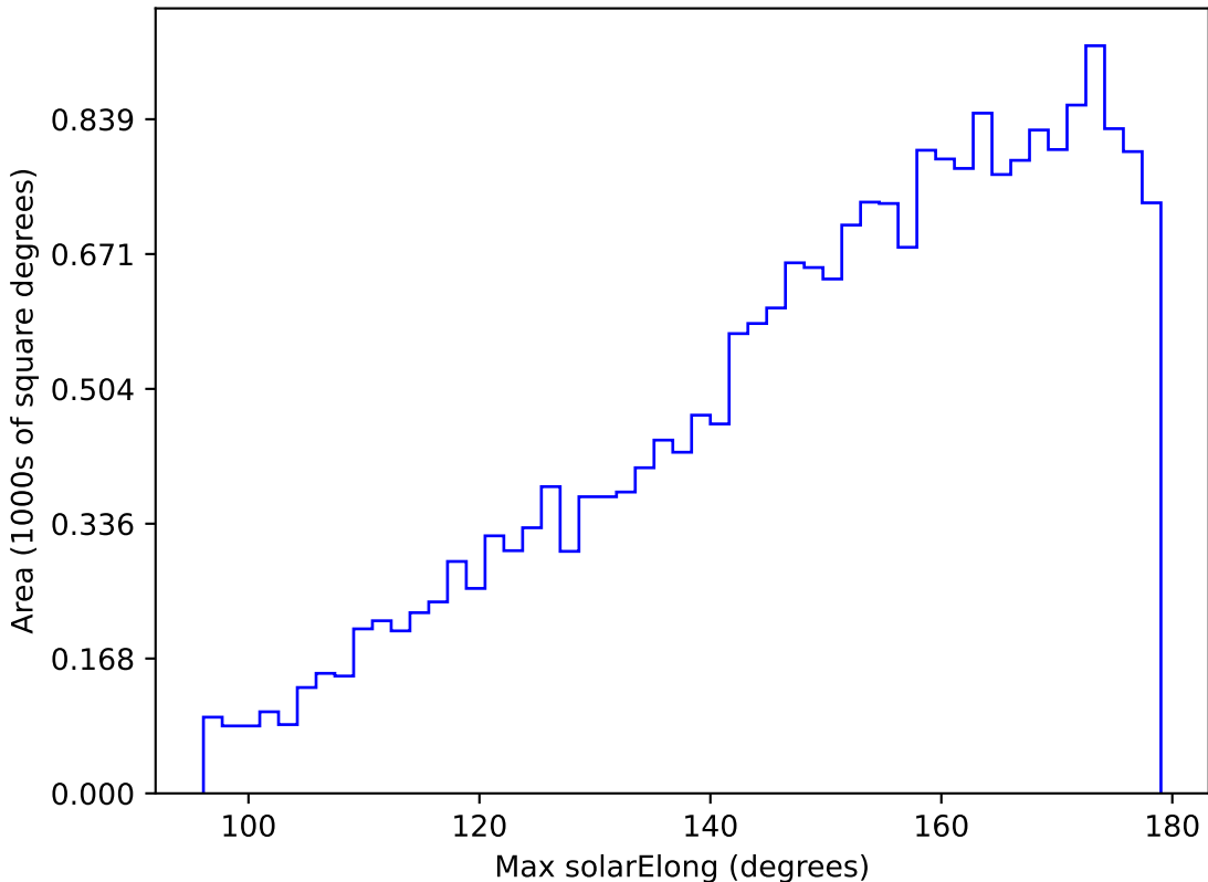
too_elab_r16_d3_griz_v3.4_10yrs All sky u band: Max solarElong
