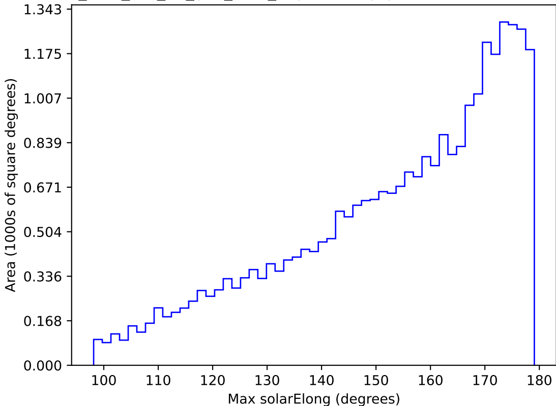
too_elab_r16_d3_griz_v3.4_10yrs All sky g band: Max solarElong
