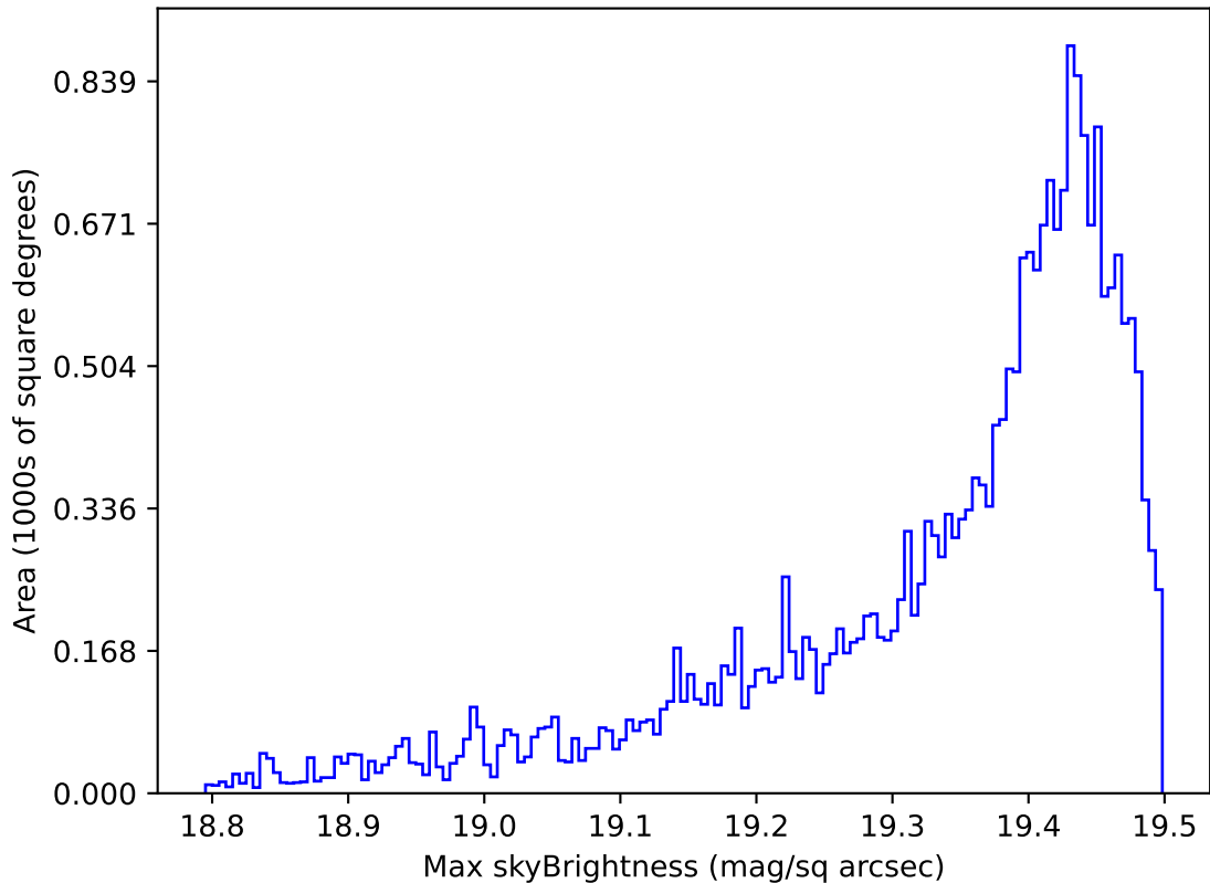
too_elab_r16_d3_griz_v3.4_10yrs Yr 1 z band: Max skyBrightness
