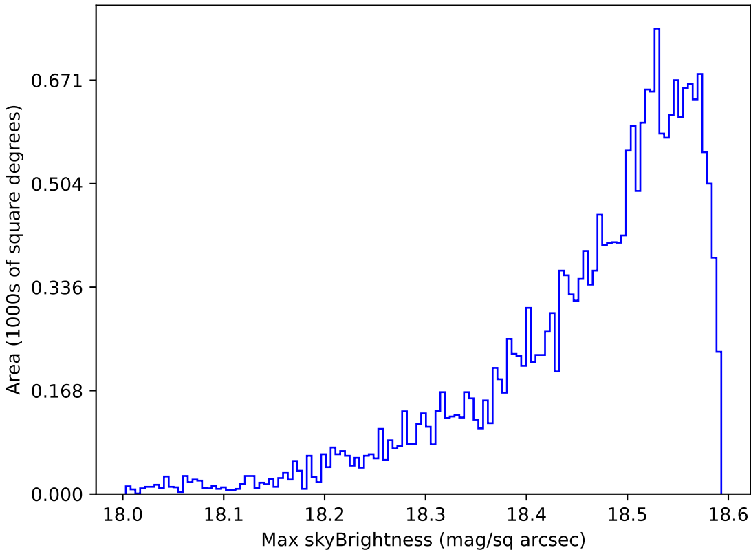
too_elab_r16_d3_griz_v3.4_10yrs Yr 1 y band: Max skyBrightness
