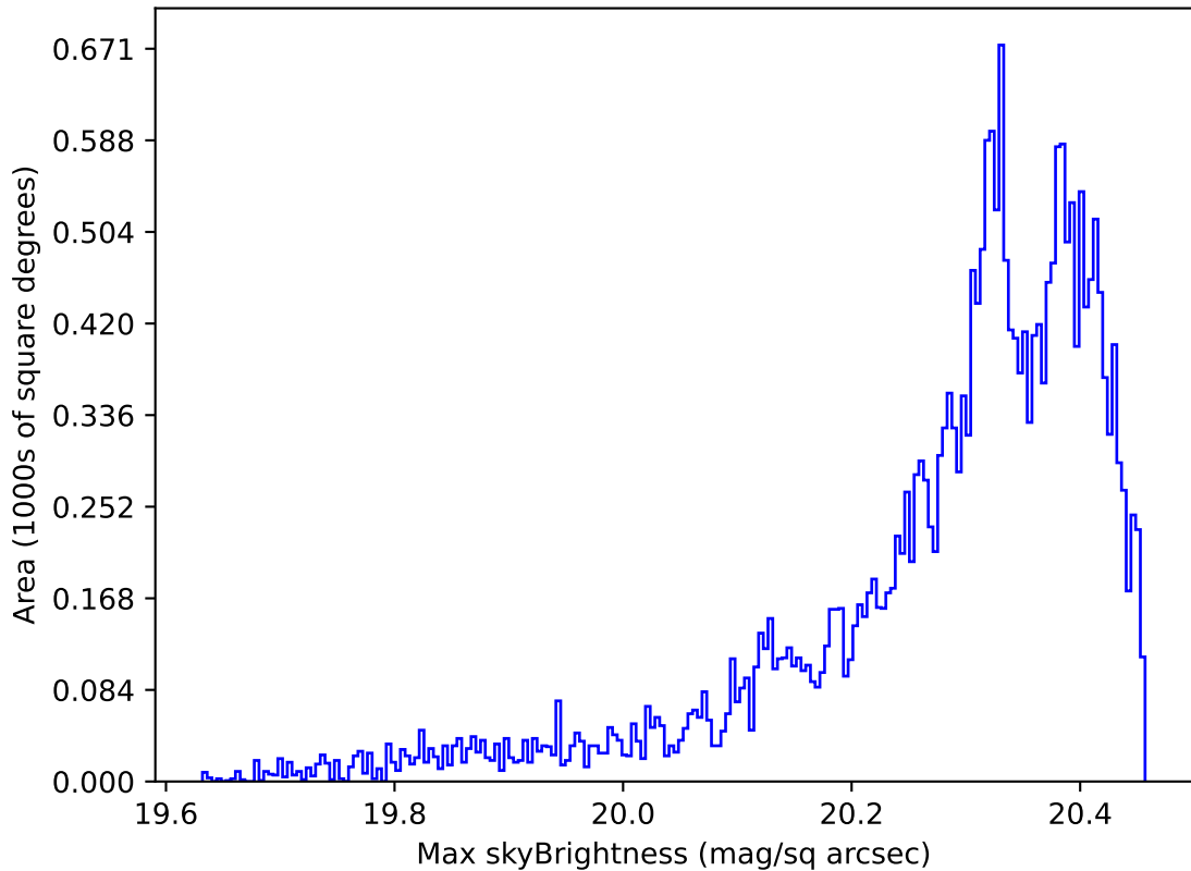
too_elab_r16_d3_griz_v3.4_10yrs Yr 1 i band: Max skyBrightness
