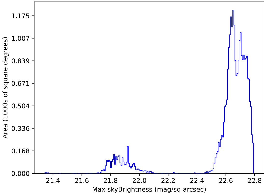
too_elab_r16_d3_griz_v3.4_10yrs Yr 1 all bands: Max skyBrightness
