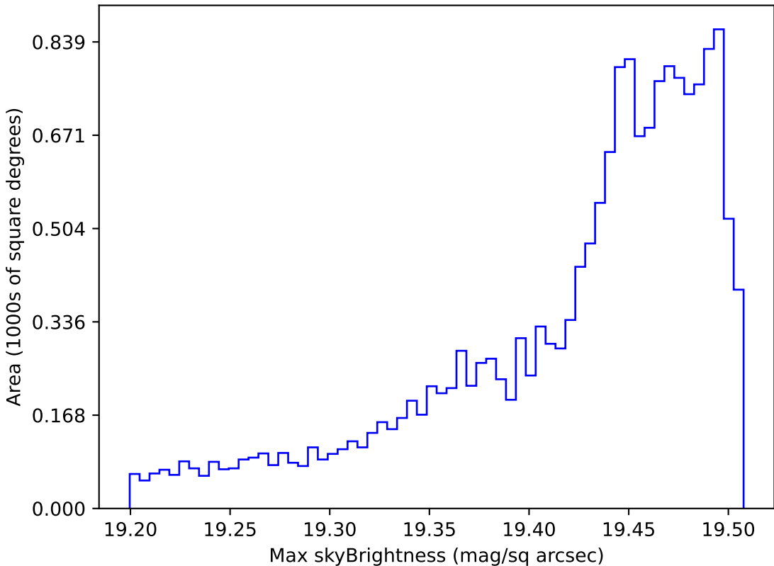
too_elab_r16_d3_griz_v3.4_10yrs WFD z band: Max skyBrightness
