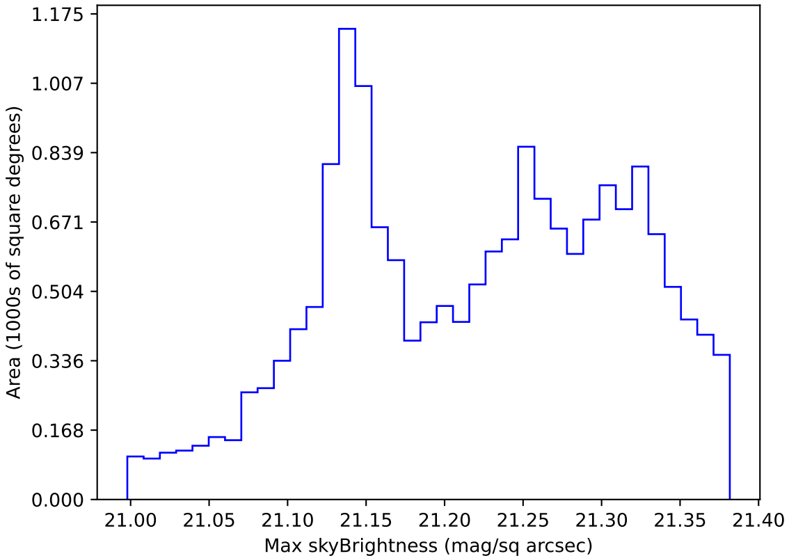
too_elab_r16_d3_griz_v3.4_10yrs WFD r band: Max skyBrightness
