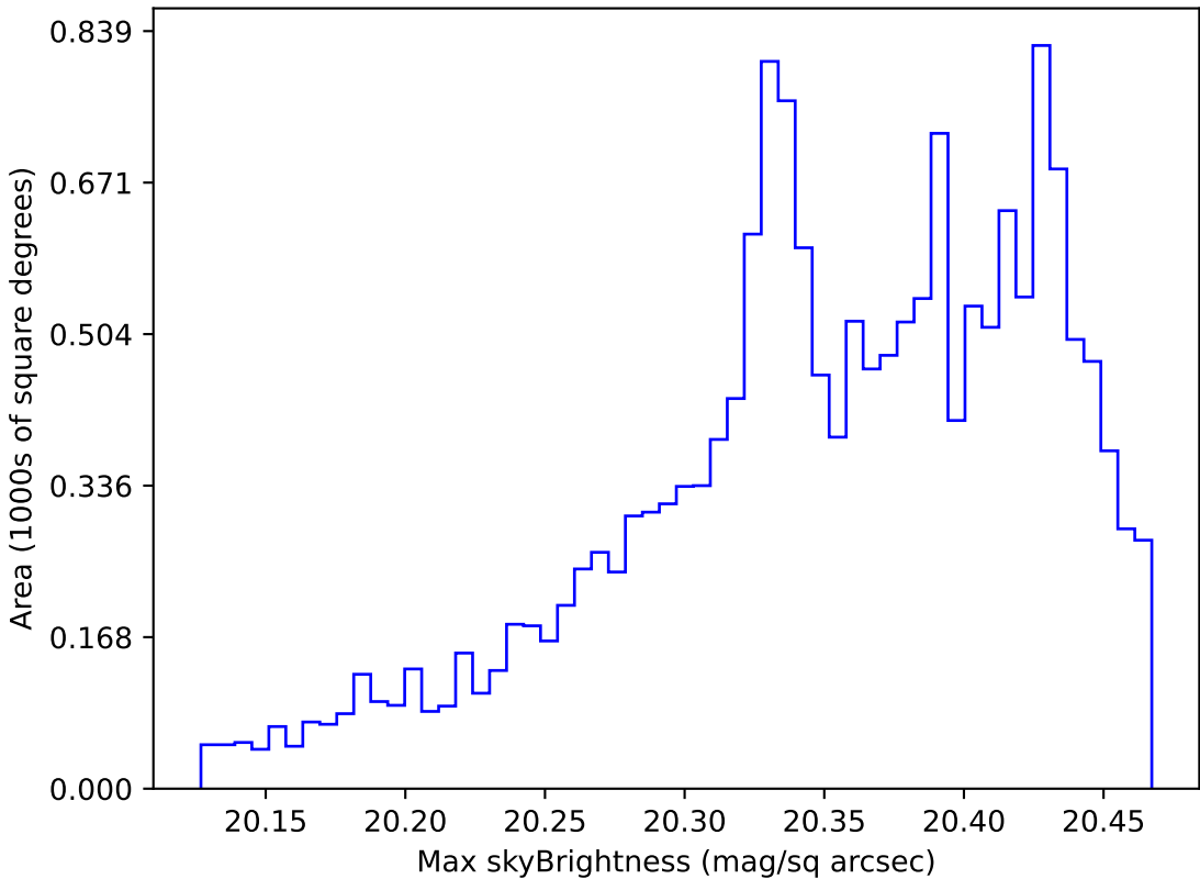
too_elab_r16_d3_griz_v3.4_10yrs WFD i band: Max skyBrightness
