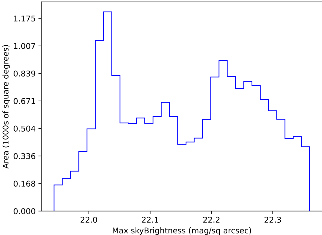
too_elab_r16_d3_griz_v3.4_10yrs WFD g band: Max skyBrightness
