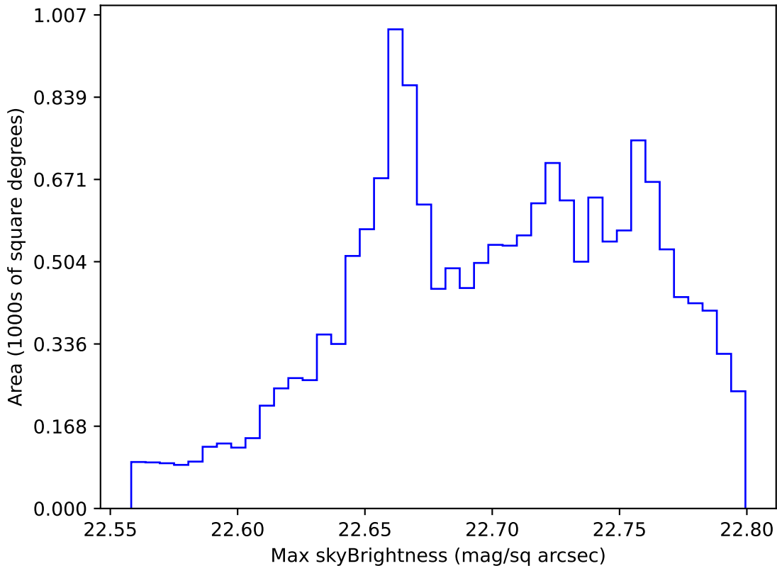
too_elab_r16_d3_griz_v3.4_10yrs WFD all bands: Max skyBrightness
