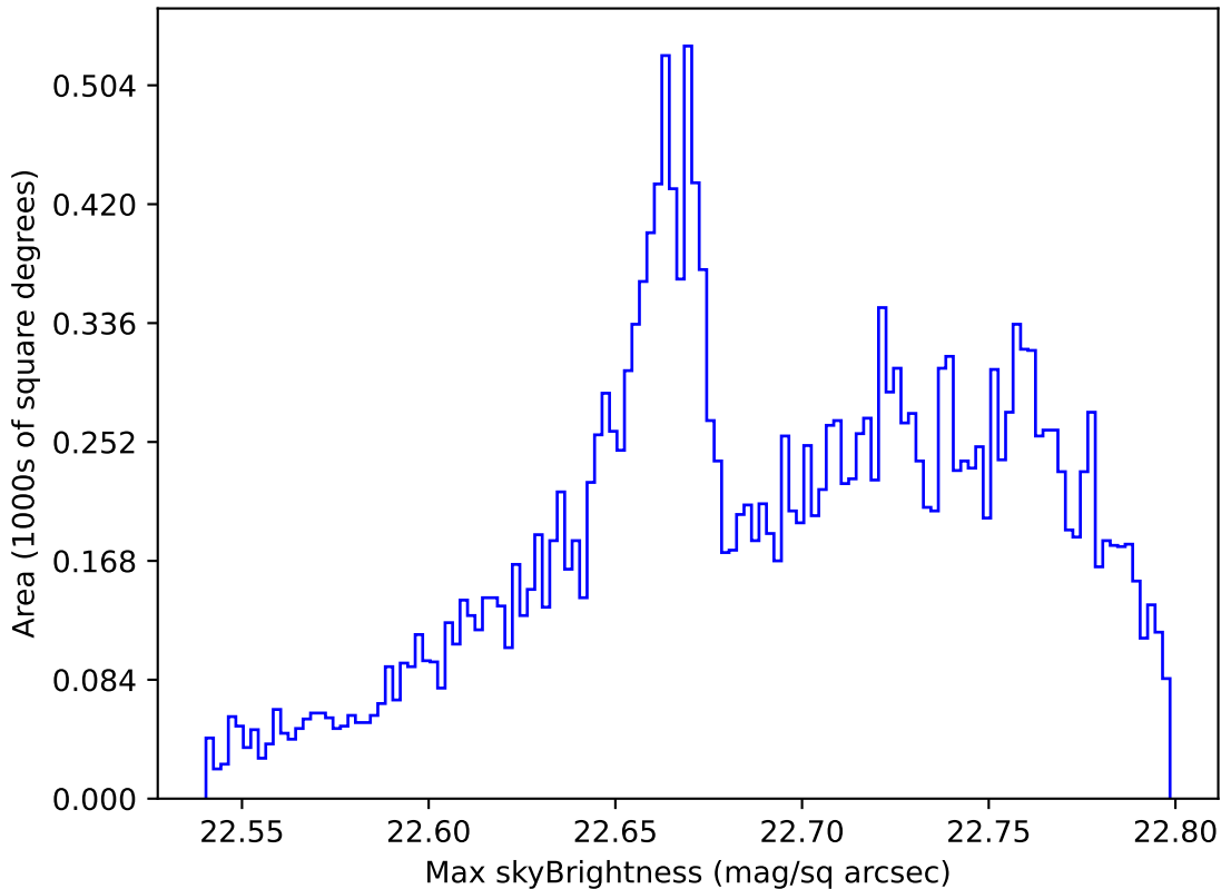
too_elab_r16_d3_griz_v3.4_10yrs All sky u band: Max skyBrightness
