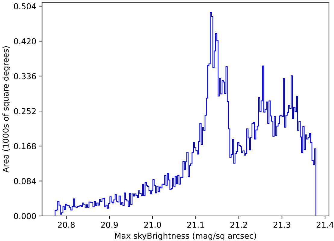
too_elab_r16_d3_griz_v3.4_10yrs All sky r band: Max skyBrightness
